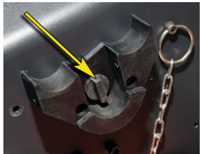
Figure 34. Driven Shaft Saddle Key.
