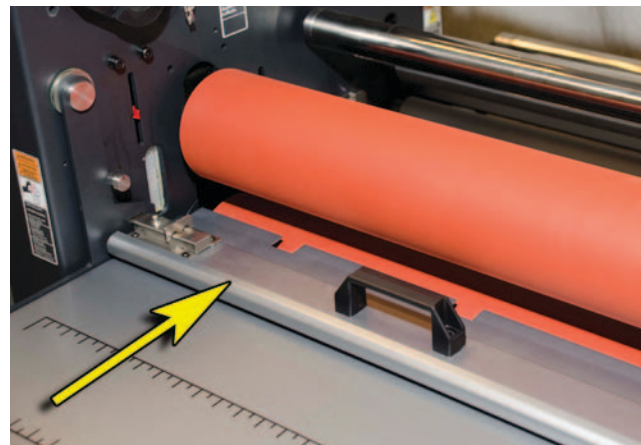
Figure 18. Pressure Plate.
