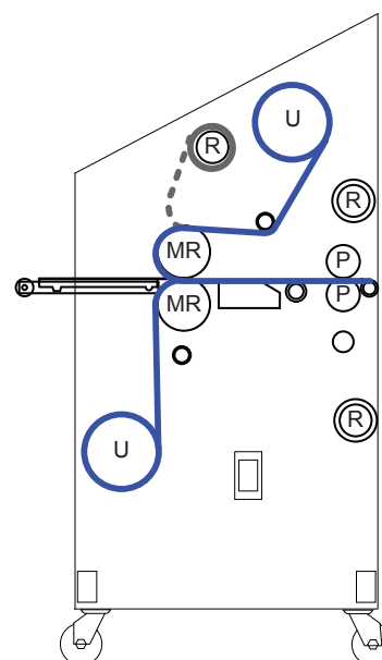
Figure 49. PSA decalling diagram.
