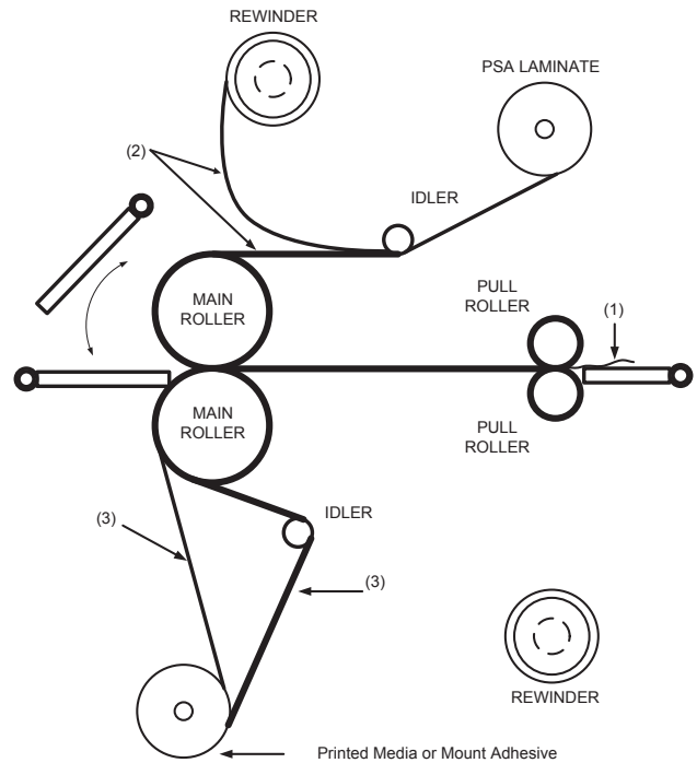
Figure 46. Cutting film from the laminator diagram.
