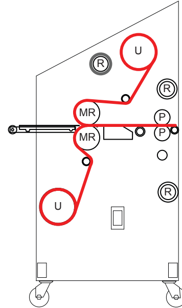
Figure 52. Thermal lamination diagram.
